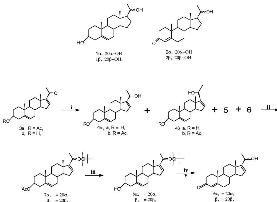
Scheme 1. (i) CeCl 3 , NaBH 4 , MeOH; or Zn, HOAc; or LTBAH, THF; or Al( i -PrO) 3 ; (ii) t -BuMe 2 SiCl, imidazole, DMF; (iii) KOH, MeOH; (iv) PTS, acetone; (v) Al( i -PrO) 3 , cyclohexanone, toluene. (5) Pregnenolone 3-acetate; (6) pregnen-3 \beta ,20 \beta -diol.
